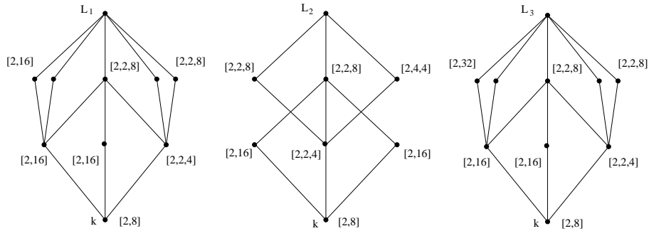
FIGURE 4. Three subfield lattices and associated 2-class groups
