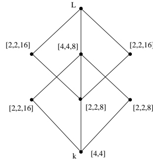
FIGURE 2. A lattice of subfields and 2-class groups
