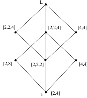
FIGURE 3. A lattice of subfields and 2-class groups
