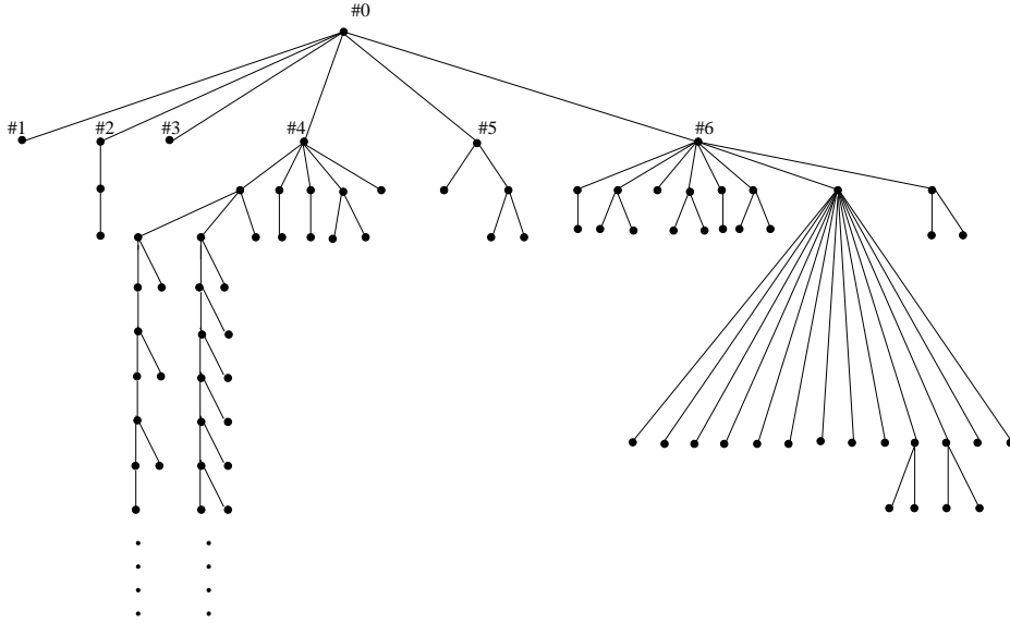
FIGURE 1. A tree of groups
